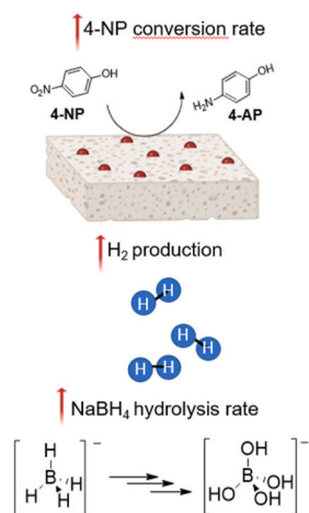
Fig. 5. Schematic reaction mechanism proposed by Grzeschik.
