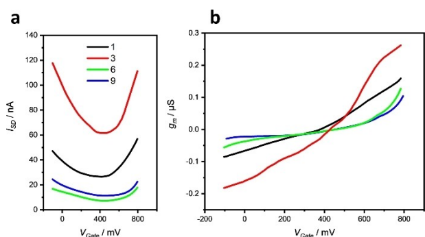
Figure 2. a) Transfer curves of rGO-FETs fabricated with different numbers of deposition pulses: 1 (black), 3 (red), 6 (green), and 9 (blue). V_{SD} = 50 mV, scan rate for V_G = 100 \text{ mV s}^{-1} . b) Transconductance ( g_m ) plots derived from (a).
