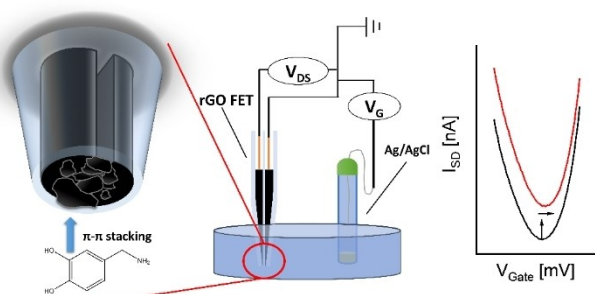
Figure 3. Electrode configuration of the measurement setup and illustration of the shift in the transfer curve of the rGO-FET upon addition of 100 \mu\text{M} DA (red curve).
