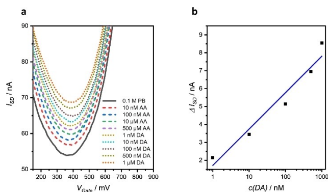
Figure 5. a) Transfer curves recorded in 0.1 m phosphate buffer, pH 7.4 upon additions of 10 nM to 500 \mu M AA (dashed lines) followed by additions of 1 nM to 1 \mu M DA (dotted lines). V_{SD} = 50 \text{ mV} , scan rate = 100 \text{ mVs}^{-1} . b) Calibration curve derived from a) showing \Delta I_{SD} at V_G = +200 \text{ mV} vs the DA concentration ( R^2 = 0.951 with a sensitivity of 2.03 \pm 0.26 \text{ nA/dec} ).
