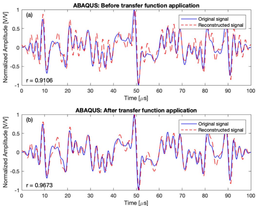
Figure 11. TR process applied to a broadband signal using the transfer function (ABAQUS TM )
