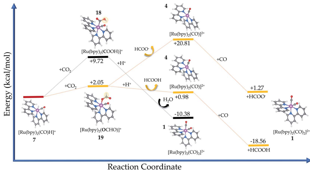
Fig. 5 Energy diagram for different pathways of CO 2 conversion with Gibbs free energies of reaction in solvated phase \Delta_r G_{(\text{soln})} (kcal mol -1 ), using the hydride complex (7) as a reference. [Ru(bpy) 2 (CO)(COOH)] + and [Ru(bpy) 2 (CO)(OCHO)] + are also referred to as C-bound (18) and O-bound species (19), respectively. In the third column, all products are still weakly bound to the Ru-complex structure, while the recovery of the starting complex (1) takes place at the third or fourth step, depending on the reaction intermediate. Color code: lilac (ruthenium), grey (carbon), blue (nitrogen), red (oxygen) and white (hydrogen).
