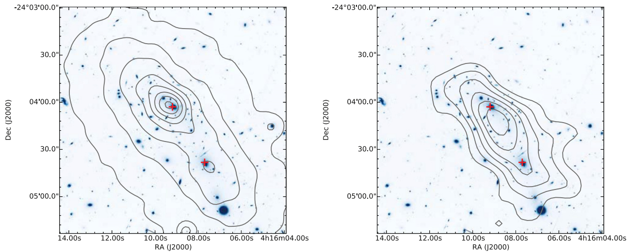
Figure 12. HST ACS/F814W optical image of MACS J0416, with overlaid Chandra (left) and JVLA (right) contours. X-ray contours are the same as in Figure 10. Radio contours are based on the JVLA image with the emission from compact sources subtracted using a Gaussian uv-taper of 20'' . The JVLA contours are drawn at [60, 80, 100, 120, 140, 160] \mu\text{J}/\text{beam} . The centers of the DM halos of the NE and SW subclusters are marked with red crosses.
