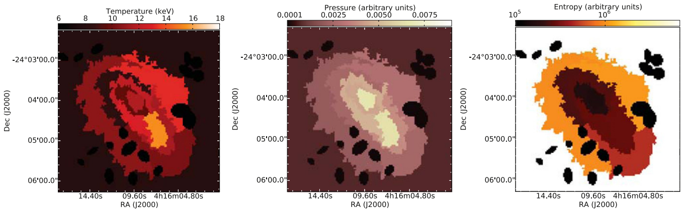
Figure 2. Temperature, pseudo-pressure, and pseudo-entropy maps of MACS J0416.1-2403. In all maps, black elliptical regions mark the regions from which point sources have been removed.
