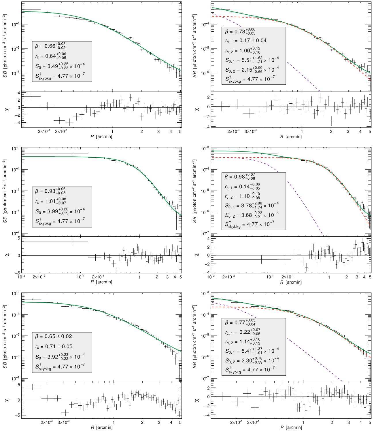
Figure 5. \beta -model (left) and double \beta -model (right) fits to the surface brightness profiles of the NE sectors with position angles of 45^\circ-115^\circ (top), 115^\circ-155^\circ (middle), and 155^\circ-225^\circ (bottom). The position angles are measured from W, in a counterclockwise direction. For all the profiles, a double \beta -model constitutes a better fit than a single \beta -model, with confidence levels of 4.4\sigma for the top profile, 3.3\sigma for the middle profile, and 6.4\sigma for the bottom profile. The individual \beta -models are shown with dashed lines. For clarity, all profiles shown have been regrouped in the plots to have 200 counts per bin. The best-fitting model parameters are listed on the plots; radii units are arcmin, and surface brightness units are \text{photon cm}^{-2} \text{s}^{-1} \text{arcmin}^{-2} . Fixed parameters are shown with a superscripted \dagger . The bottom panel shows the residuals of the fit.
