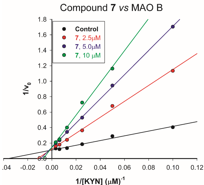
Figure S1 Double reciprocal plots of MAO B activity in the presence of various concentrations of compound 7. Continuous lines are the results of the linear regression analysis of the plotted data ( r > 0.99 )
