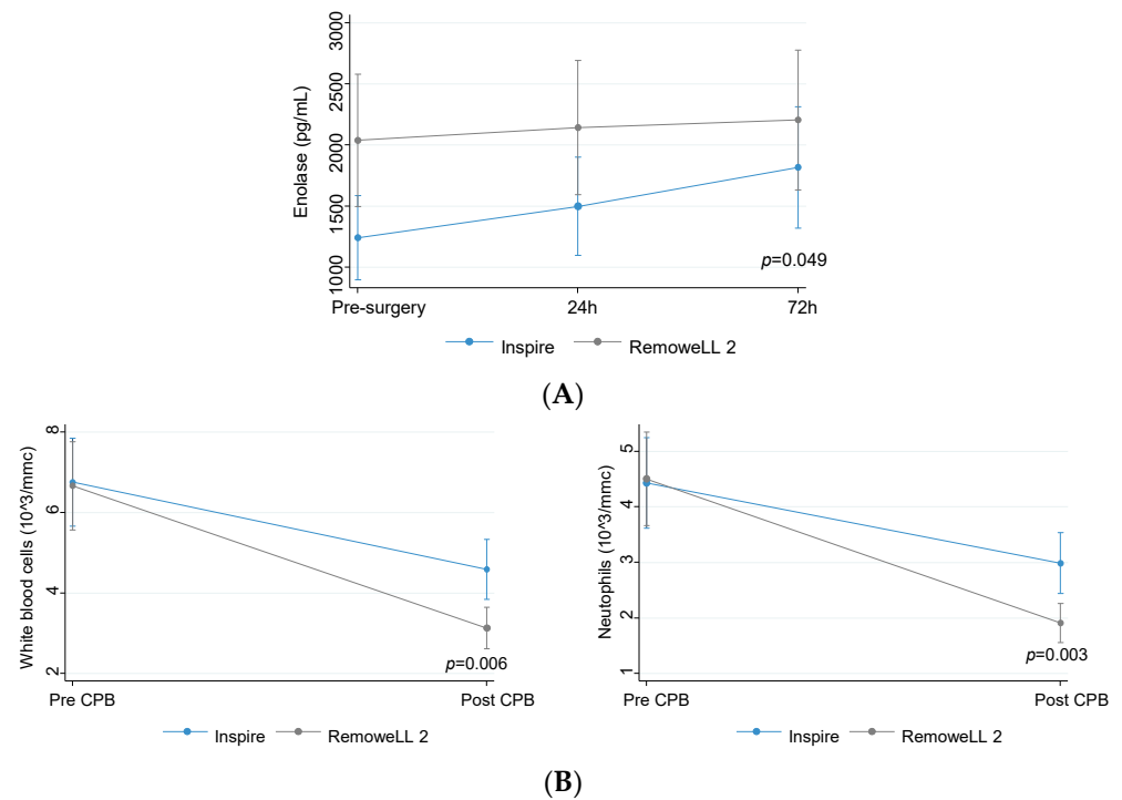
Figure 3. (A) Levels of enlase (predicted values and confidence intervals) in patients assigned to Inspire ( n = 73 ) or RemoweLL 2 ( n = 81 ) oxygenator; (B) levels of blood leukocytes in patients assigned to Inspire ( n = 73 ) or RemoweLL 2 ( n = 81 ) oxygenator. Total blood leukocytes (predicted values and confidence intervals) (left panel), neutrophils (predicted values and confidence intervals) (right panel).
