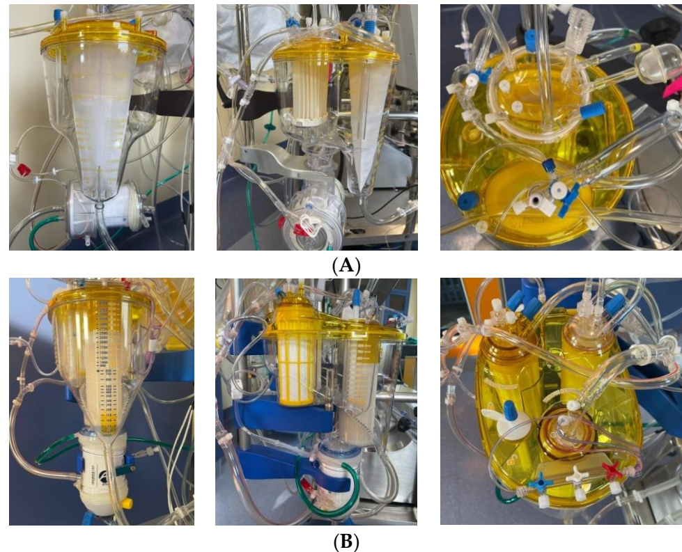
Figure 1. RemoweLL 2 and Inspire oxygenators. (A) Inspire: frontal view, lateral view with filter detail, chamber top view; (B) RemoweLL 2: frontal view; lateral view with filter detail; dual chamber top view.
