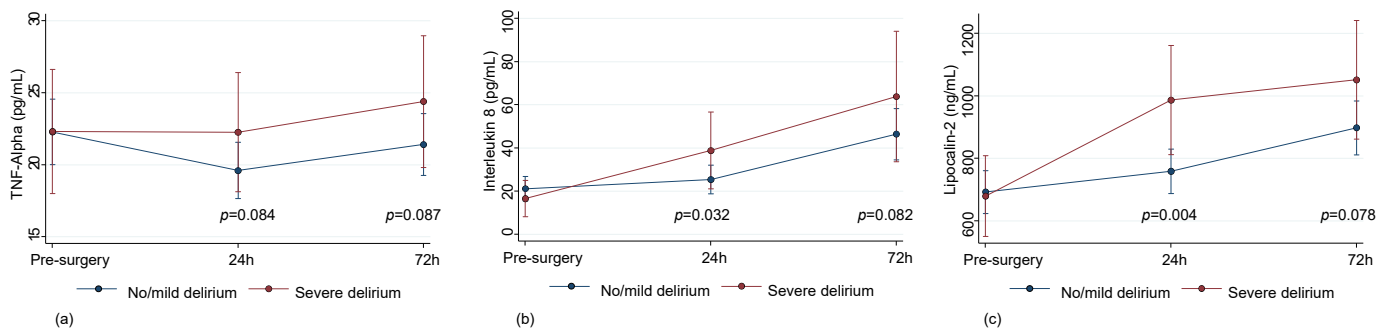
Figure 4. Levels of inflammatory markers in patients with no/mild ( n = 122 ) or severe ( n = 32 ) delirium. Plasma levels of TNF \alpha (predicted values and confidence intervals) (a); Plasma levels of Interleukin 8 (predicted values and confidence intervals) (b); Plasma levels of Lipocalin-2 (predicted values and confidence intervals) (c).
