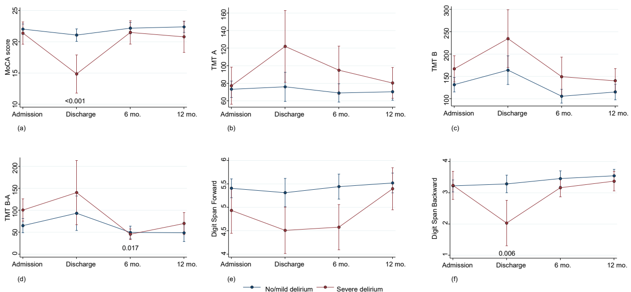
Figure 2. Cognitive decline according in patients with no/mild ( n = 122 ) or severe ( n = 32 ) delirium: Montreal Cognitive Assessment (MoCA) score (a); Trail Making Test (TMT) A (b); TMT B (c); TMT B-A (d) Digit Span Forward (e); Digit Span Backward (f). Values are predicted values and confidence intervals.
