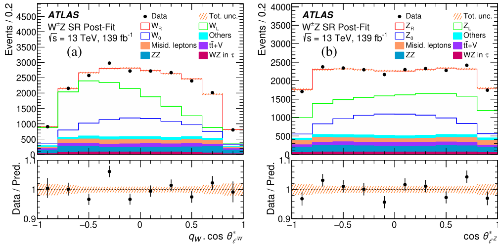
Fig. 3. Post-fit distributions of (a) q_W \cdot \cos \theta_{\ell^*}^W and (b) \cos \theta_{\ell^*}^{Z^*} in W^\pm Z events at detector level in the signal region (SR). Respective contributions of the W^\pm Z individual helicity states 0, L and R of the W and Z bosons and backgrounds are normalised to the expected number of events after the fit. The sum of background events containing misidentified leptons is labelled ‘Misid. leptons’. The sum of VVV , WZjj-EW and tZj background events is labelled ‘Others’. The uncertainty band around the expectation includes all systematic uncertainties as obtained from the fit.
