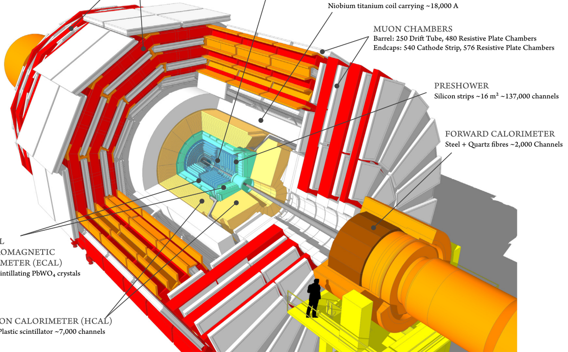
Fig. 2. The CMS detector for the data-taking period 2017–2018.
