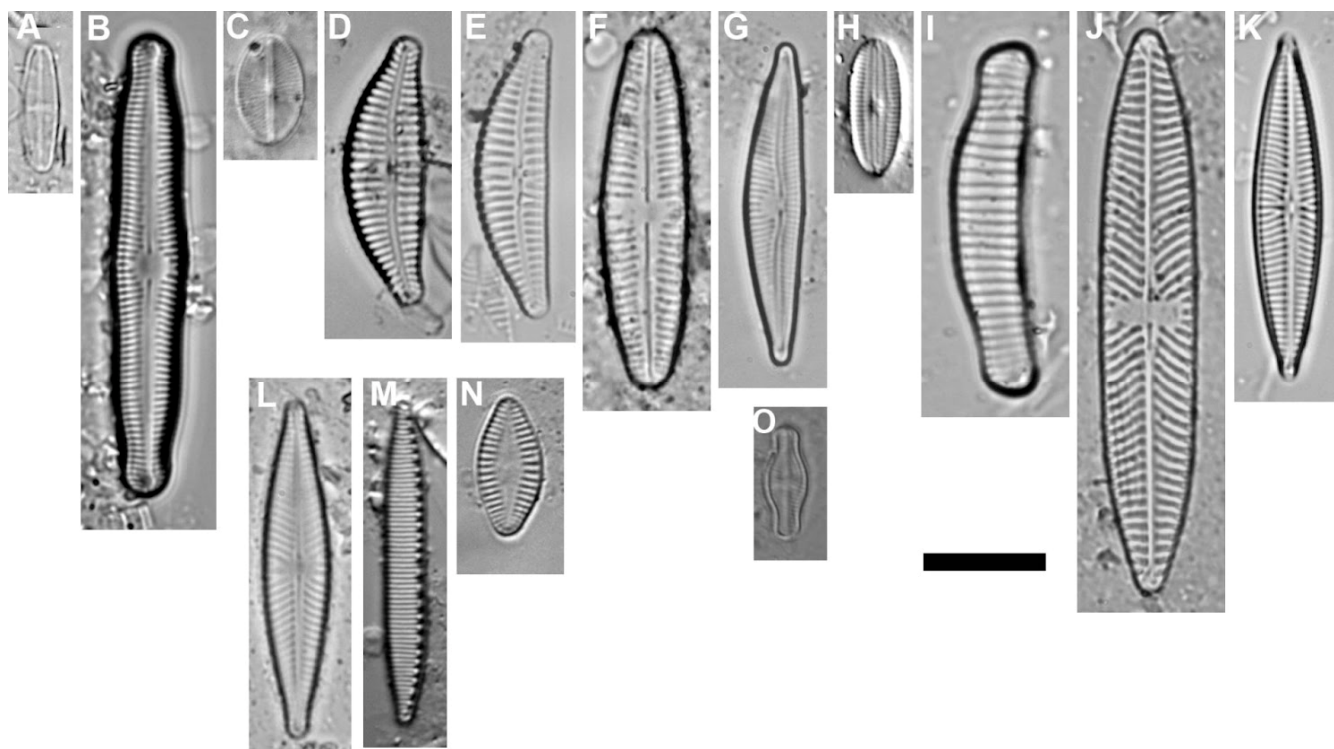
Figure 4. Micrographs of characteristic, rare, and Red-List species. (A) Achnanthydium dolomiticum , (B) Caloneis tenuis , (C) Cavinula jaernefeltii , (D) Cymbella affinis , (E) Cymbella tridentina , (F) Cymboplectura subaequalis , (G) Delicata delicatula , (H) Diploneis petersenii , (I) Eunotia arcubus , (J) Navicula dealpina , (K) Navicula subalpina , (L) Navicula wildii , (M) Nitzschia alpina , (N) Platessa montana , (O) Sellaphora sp. aff. schadei . (B,H,M) = Nomarski (DIC); all the other bright field. Scale bar 10 \mu m.
