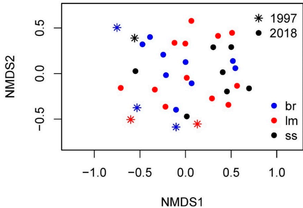
Figure 8. Ordination of samples using Nonmetric Multidimensional Scaling of all the samples. br = bryophytes (epiphytic), lm = lithic material (epilithic), ss = surface sediments (epipellic).
