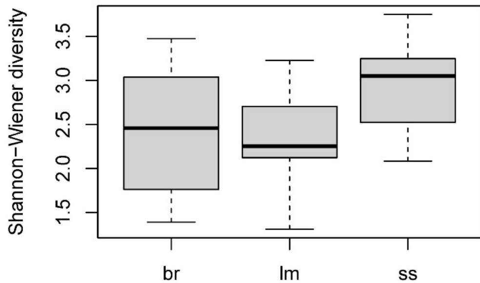
Figure 9. Boxplot of the Shannon-Wiener diversity of diatoms using as groups the substrates (br = bryophytes, lm = lithic material, ss = surface sediments).
