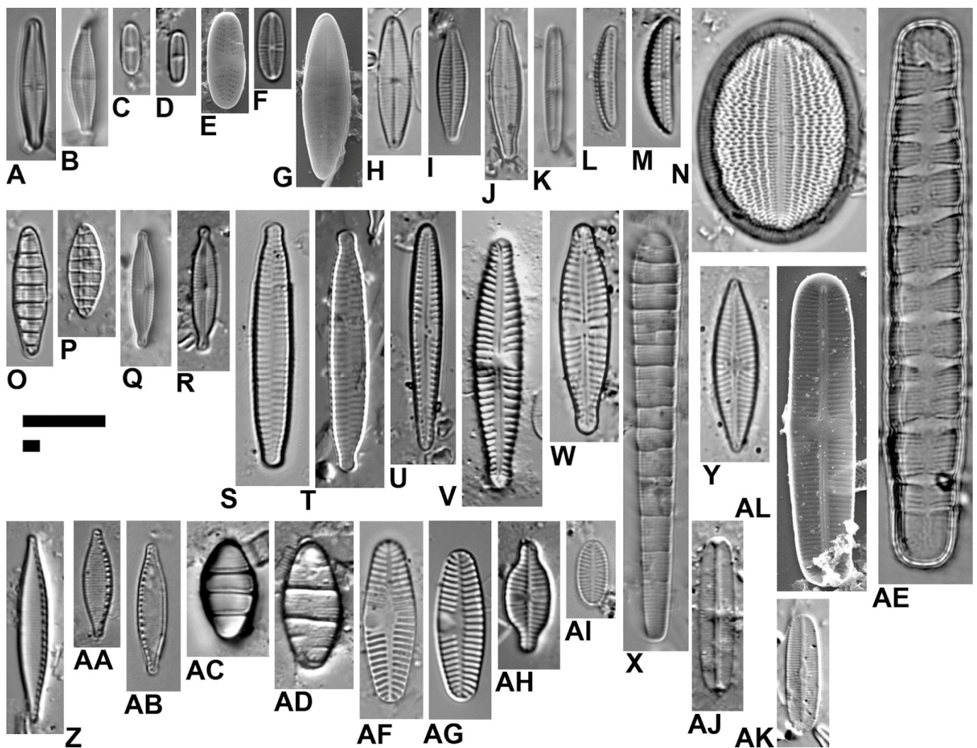
Figure 3. Micrographs of the most frequent and abundant species. (A) Achnanthydium minutissimum , (B) Achnanthydium jackii , (C–E) Achnanthydium lineare , (F) Achnanthydium pfisteri , (G,H) Achnanthydium pyrenaicum , (I,J) Achnanthydium rostrropyrenaicum , (K) Achnanthydium sublineare , (L) Amphora micra , (M) Amphora pediculus , (N) Cocconeis lineata , (O,P) Denticula tenuis , (Q,R) Encyonopsis krammeri , (S,T) Fragilaria pectinalis , (U) Gomphonema elegantissimum , (V,W) Gomphonema micropus , (X) Meridion circulare , (Y) Navicula cryptotenella , (Z)—(AA) Nitzschia fonticola , (AB) Nitzschia perminuta , (AC,AD) Odontidium mesodon , (AE) Odontidium neomaximum , (AF,AG) Planothidium lanceolatum , (AH) Planothidium reichardtii , (AI) Psammothidium grischunum , (AJ,AL) Rossithidium petersenii . (E,G,AL) = SEM; (D,I,P,R,T,V,Z,AD,AG,AH,AJ,AK) = Nomarski (DIC); all the other bright fields. Scale bars: long (LM) 10 \mu m; short (SEM) 1 \mu m.
