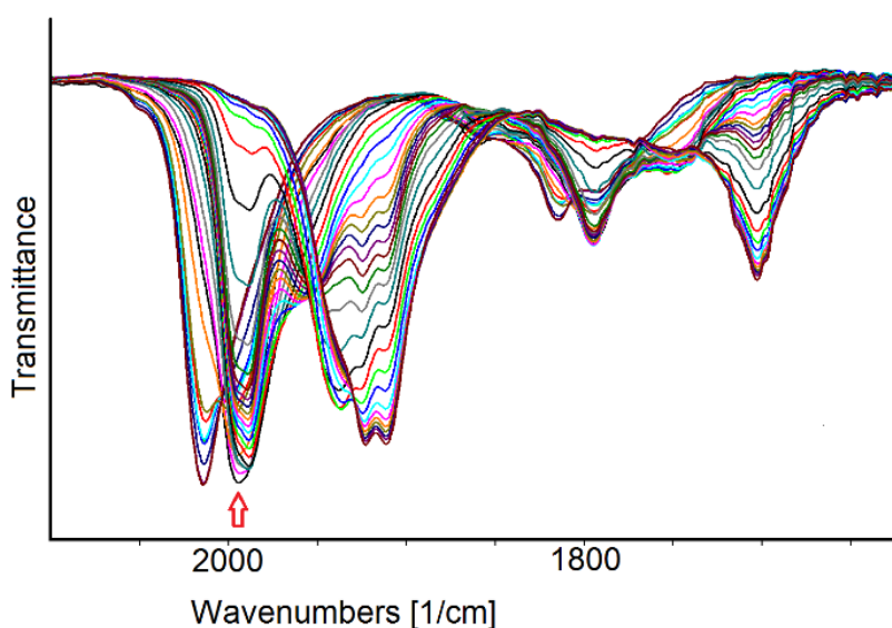
Figure 9. Infrared spectra of [\text{Rh}_{12}\text{Sn}(\text{CO})_{27}]^{4-} recorded in an OTTE cell during the progressive decrease of the working electrode potential E from +0.2 to -1.9 V ( vs Ag pseudo reference electrode) in \text{CH}_3\text{CN} containing 0.1 \text{ mol dm}^{-3} [\text{N}^t\text{Bu}_4][\text{PF}_6] . The absorptions of the solvent and supporting electrolyte have been subtracted. The red arrow indicates the initial spectrum.
