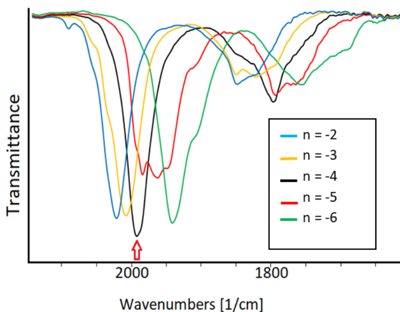
Figure 8. Selected infrared spectra of [\text{Rh}_{12}\text{Ge}(\text{CO})_{27}]^n as a function of the cluster charge n in \text{CH}_3\text{CN} containing 0.1 \text{ mol dm}^{-3} [\text{N}^t\text{Bu}_4][\text{PF}_6] . The absorptions of the solvent and supporting electrolyte have been subtracted.
