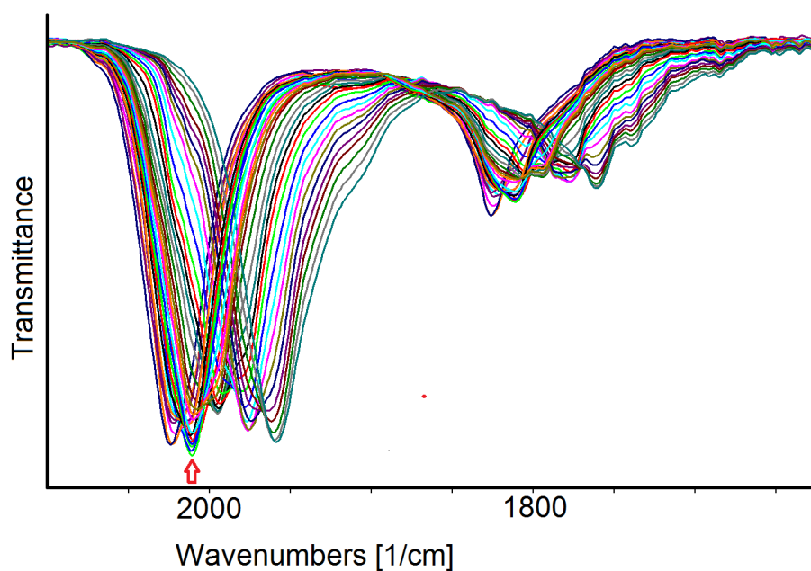
Figure 2. Infrared spectra of [\text{Rh}_{12}\text{Sb}(\text{CO})_{27}]^{3-} recorded in an OTTLE cell during the progressive decrease of the working electrode potential E from +0.3 to -1.6 V( vs Ag pseudo reference electrode) in \text{CH}_3\text{CN} containing 0.1 \text{ mol dm}^{-3} [\text{N}^+\text{Bu}_4][\text{PF}_6^-] . The solvent and supporting electrolyte absorptions have been subtracted. The red arrow indicates the initial spectrum.
