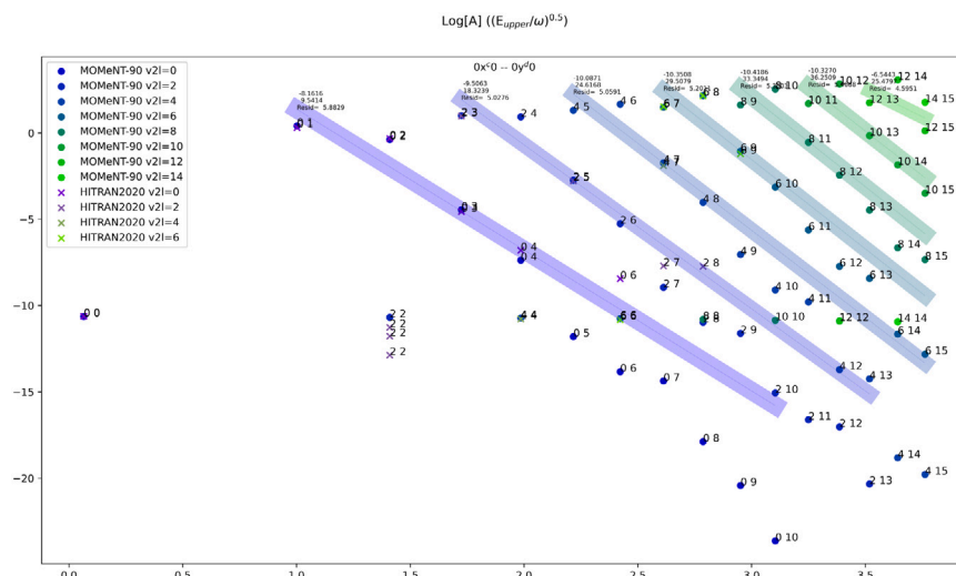
Fig. 20. Demonstration of the NID on the 0x^0 - 0y^d series of transitions of HCN with HITRAN2020 and HITRAN2024 (MOMeNT-90) line lists.
