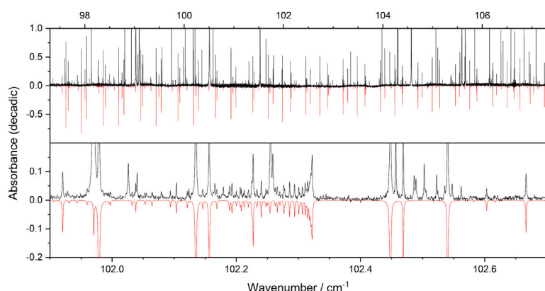
Fig. 25. Top panel: Experimental (upward; 0.25 Torr) and simulated (downward) spectra of \text{H}^{13}\text{COOH} using a Gaussian FWHM of 0.0006\text{ cm}^{-1} . Bottom panel: Experimental (upward; 1.5 Torr) and simulated (downward) spectra using a Lorentzian FWHM of 0.0012\text{ cm}^{-1} .
