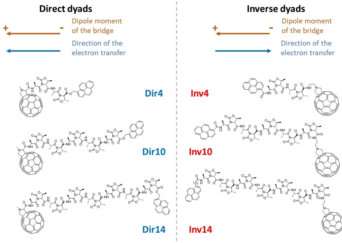
Figure 1. Engineering of the D- \gamma -A dyads. Sketched molecular structures of the six D- \gamma -A dyads synthesized in this work. The Py unit acts as an electron donor (D) and the C 60 unit as an electron acceptor (A). Different chiral bridges have been probed to investigate the role of the bridge length and its electric dipole moment. Legend: Dir = direct dyad, i.e., the electric dipole moment of the bridge is parallel to the direction of ET; Inv = inverse dyad, i.e., the electric dipole moment of the bridge is antiparallel to the direction of ET; n = number of amino acids of the peptide bridge.
