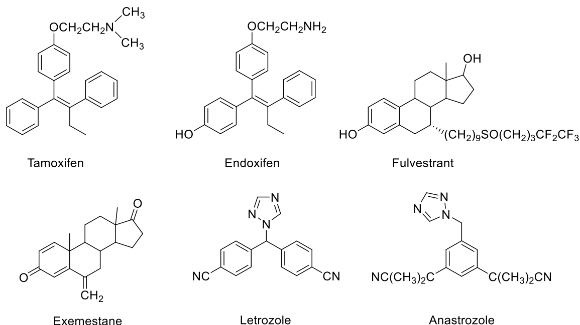
Figure 1. Molecular structures of selective estrogen receptor modulators (SERMs, Tamoxifen and its metabolite Endoxifen) and degraders (Fulvestrant), along with the third-generation aromatase inhibitors (AIs, Exemestane, Letrozole and Anastrozole).
