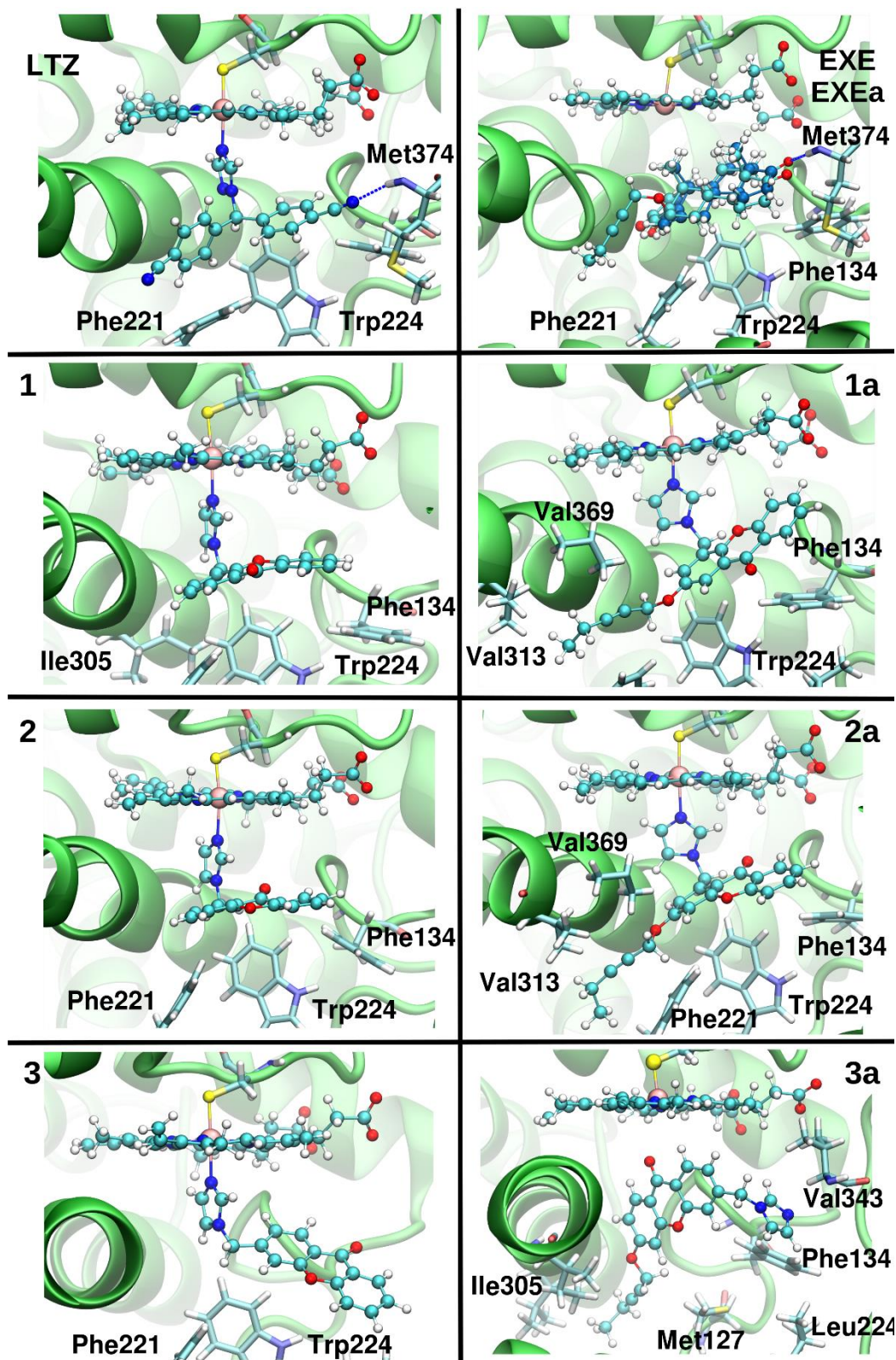
Figure 5. Representative structures as obtained from quantum-classical molecular dynamics simulations of letrozole (LTZ), exemestane (EXE) and its derivative (EXEa), 22 compounds 1-3 and 1a-3a . For comparison, the dual mode steroidal inhibitor EXEa is also reported superimposed to EXE. The inhibitors and the heme moiety are shown in a ball and stick representation, while hydrophobic residues involved in stacking and hydrophobic interactions are highlighted as sticks. When present, hydrogen bonds are shown as dashed red and blue lines.
