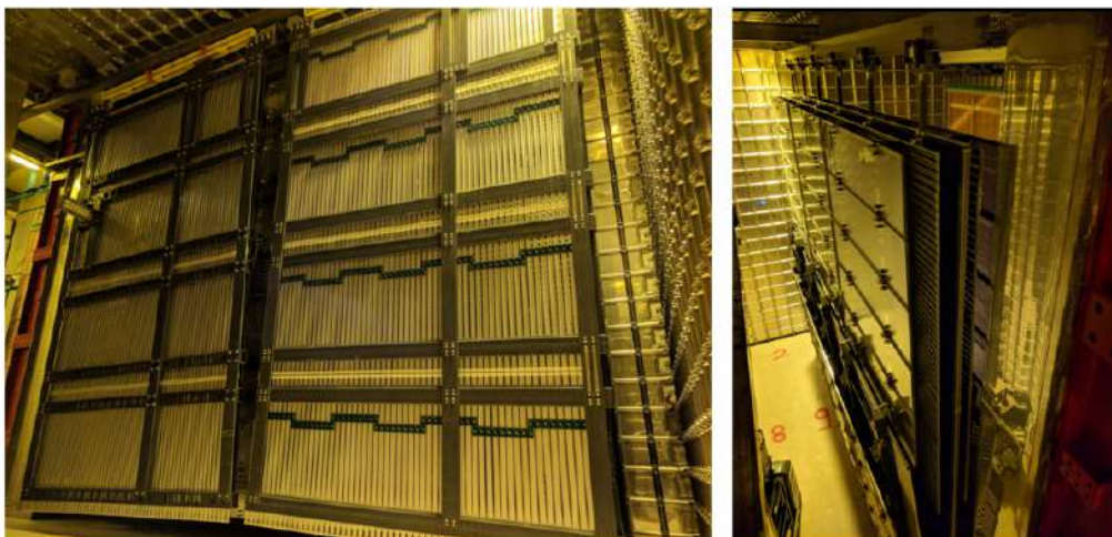
Figure 76. . Left: salève-side drift FC end-walls are ready to be deployed inside the cryostat. Right: CPA and FC assemblies inside the cryostat ready to be pushed to their final position.
