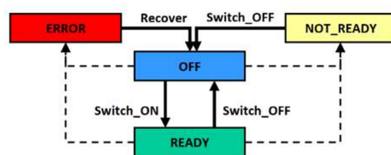
Figure 85. FSM flow diagram for turning ON/OFF a detector component.
