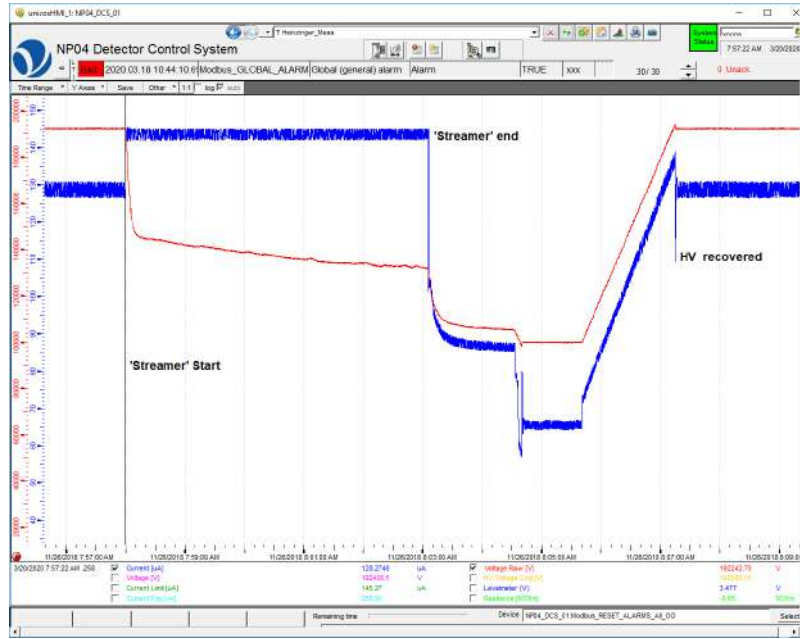
Figure 26. Automatic Recovery of a ‘streamer’ event recorded on 26/11/2018 by DCS. The HV current (in blue) is limited at 142\ \mu\text{A} ; the voltage (in red) decreases until the discharge is finished, returning to the nominal voltage after a predefined time.
