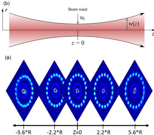
Fig. 53. Effect of an axial translation on the ring lattice potential. (a) Ring lattice intensity distribution measured at various positions along the beam propagation axis around the focal plane ( Z=0 ). Note that the initial beam, phase modified by the SLM, is not Gaussian any more. The optical potential remains undisturbed by a translation of 2.2 times the ring-lattice radius centered around the focal plane ( Z=0 ). Here R designates the ring-lattice radius of 87.5 \mu\text{m} . (b) This is in contrast to a Gaussian laser beam which exhibits a marked dependence on the axial shift from the focal plane where the beam waist w(z) scales with \sqrt{1 + (z/z_0)^2} and Rayleigh range z_0 . Reprinted with permission from Amico et al. , Sci. Rep. 4 , 4298 (2014). Copyright 2014, Author(s) licensed under a Creative Commons Attribution 4.0 License.
