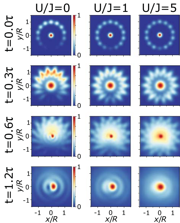
Fig. 46. Density of expanding atoms at times t = 0, 0.3\tau, 0.6\tau, 1.2\tau , with \tau = mR\sigma_r/\hbar . From left to right: U=0, U/J=1, U/J=5 . Flux \Omega = \frac{1}{2} at the degeneracy point. At intermediate time, we observe some spiral-like structure at the edges. This is not the interference with the central condensate, but a residue of the ring lattice interfering with itself. Calculated using Bose–Hubbard model, no interaction during expansion. Data in color and normalized to one. Ring has 7 particles, M = 14 ring sites, ring radius R . Width of central and ring cloud is \sigma_r = 2R/L and potential barrier \Lambda = J , 25% of atoms in central condensate. Barrier at x=0, y=-R . Reprinted with permission from Haug et al. , Phys. Rev. A 97 , 013633 (2018). Copyright 2018, American Physical Society.
