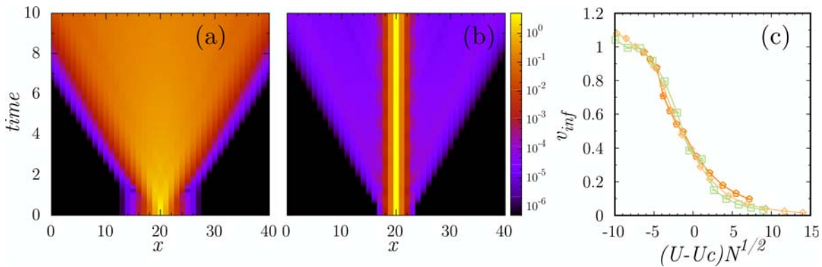
FIG. 76. Panels (a) and (b): expansion of a soliton composed by N = 5 particles, pinned to the center of a chain with L = 41 sites for interactions U = 0.4 and U = 1.8 . Panel (c): asymptotic expansion velocity v_\infty as a function of U - U_c(N) and of (U - U_c(N))\sqrt{N} .
