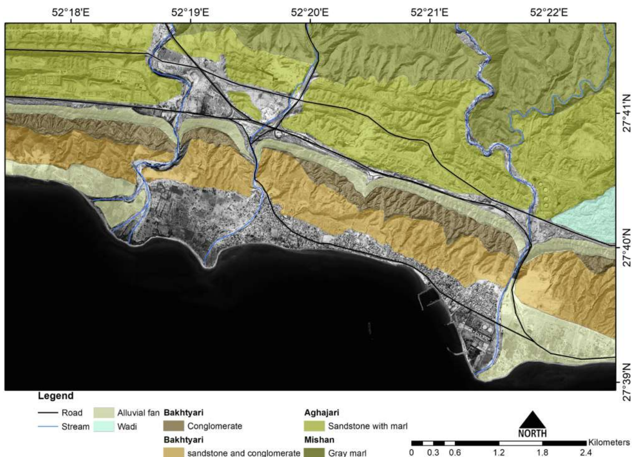
Fig. 2. Geological and geomorphological map of the Siraf watershed. The background image derives from Google Earth Pro and shows the ancient urban fabric in July 2018. Most of the historic sectors have been destroyed with the exception of some coastal quarters at risk from coastal erosion.
