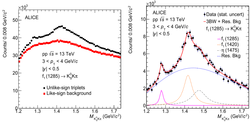
Fig. 1. Like- and unlike-sign (left) and the like-sign-subtracted (right) invariant mass distribution of K_S^0 K \pi triplets in |y| < 0.5 in minimum-bias pp collisions at \sqrt{s} = 13 TeV. The subtracted distribution is fitted with the function defined by Eq. (1), and the dotted blue line describes the residual background distribution, which is given by Eq. (2).
