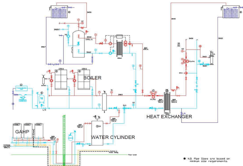
Fig. 2. Schematic Layout of Heating System in Hale Court North.
