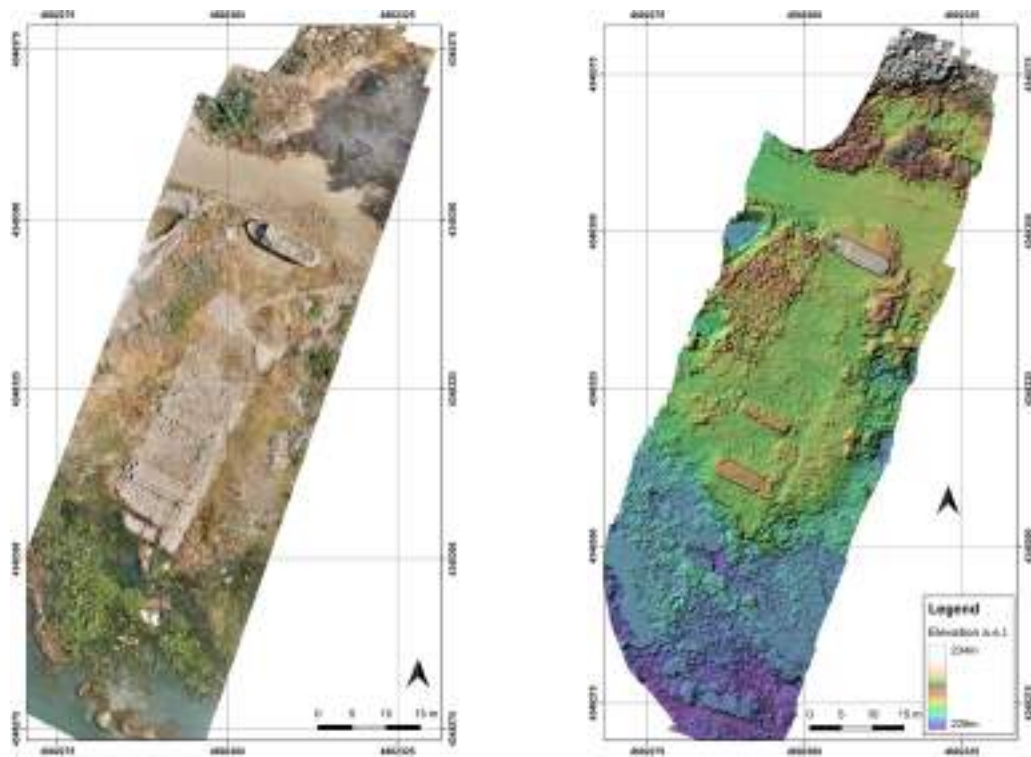
2. Orthophotomodel (left) and DSM (right) of the Old Bridge area.
