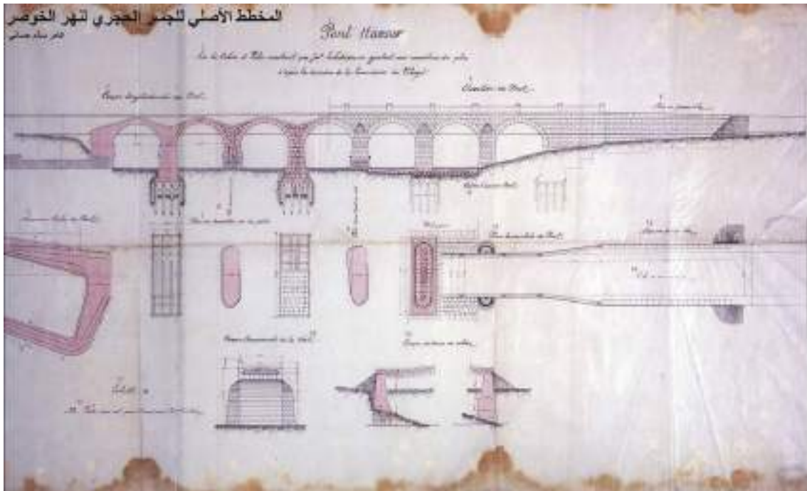
1. Architect's drawing of lower Khosr bridge, c. 1908. Constructed by G[?]. Eutychedes. Mosul Inspectorate of the State Board of Antiquities and Heritage.
