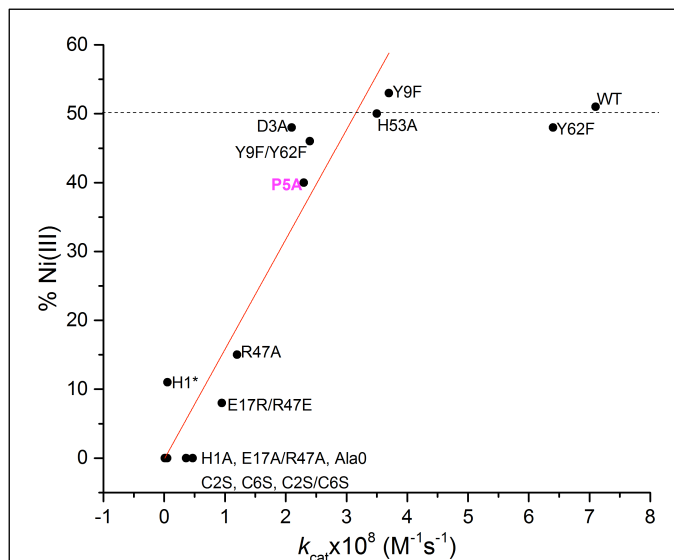
Figure 6. Relationship between the amount of Ni(III) observed in ‘air oxidized’ as-isolated samples and k_{\text{cat}} observed at pH 7.5 (see Table SI-2 for values). The red line represents a least-squares fit to the data excluding Y62F- and WT NiSOD; y = a + bx , where a = -0.18 and b = 15.9 , and R = 0.89 .
