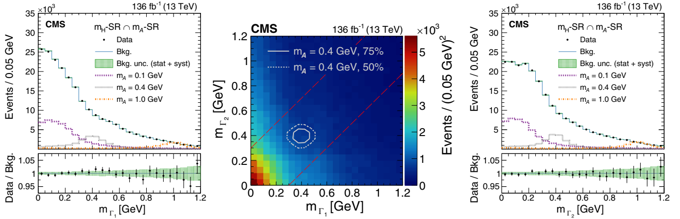
FIG. 1. Mass distributions from selected events in data. Center: the 2D- m_{\Gamma} distribution for data events in the m_{H\text{-SR}} . The red dashed lines indicate the m_{\mathcal{A}\text{-SR}} boundaries. The contours of simulated H \rightarrow \mathcal{A}\mathcal{A} \rightarrow 4\gamma events for m_{\mathcal{A}} = 0.4 GeV are plotted for 75% (solid contour) and 50% (dotted contour) of the distribution maximum. The corresponding m_{\Gamma_1} (left) and m_{\Gamma_2} (right) projections for the overlap of the m_{H\text{-SR}} and m_{\mathcal{A}\text{-SR}} are also shown. The data distributions (black points) are plotted against the total predicted background distributions (blue curves). The statistical uncertainties in the former are negligible and the total uncertainties in the latter are barely visible as green bands. The spectra of simulated H \rightarrow \mathcal{A}\mathcal{A} \rightarrow 4\gamma events for m_{\mathcal{A}} = 0.1 (purple dashed curve), 0.4 (gray dotted curve), and 1.0 GeV (orange dash-dotted curve) are also provided. They are each normalized to the value of \mathcal{B}(H \rightarrow \mathcal{A}\mathcal{A} \rightarrow 4\gamma) that is expected to be excluded by the background model (described under the CL_s criterion in our results) times 10^3 . The black points in the lower panels of the left and right plots give the ratios of the data to the predicted background distributions. The vertical bars represent the statistical uncertainties in the former, and the green bands represent the total uncertainty in the latter.
