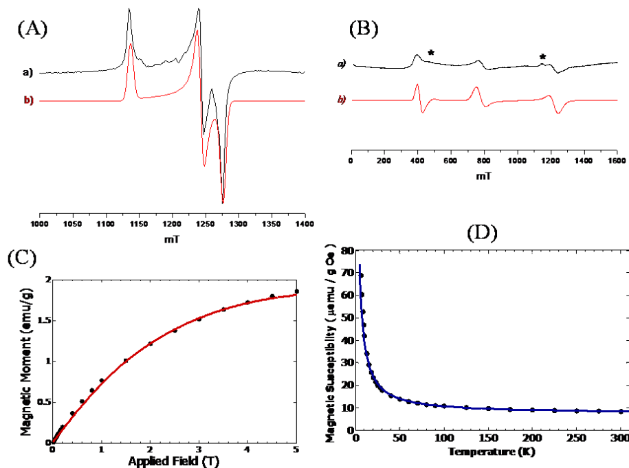
Fig. 8. EPR spectra in solid at 5 K of [\text{Co}_8\text{Pt}_4\text{C}_2(\text{CO})_{24}]^{n-} : (a) n = 1 , S = 1/2 ; (b) n = 2 , S = 1 (* background impurity) Experimental spectra in black, simulated spectra in red. (c) First magnetization curve at 2 K and (d) temperature dependence of magnetization of [\text{Co}_8\text{Pt}_4\text{C}_2(\text{CO})_{24}]^{2-} . Reproduced with permission from ref. 89.
