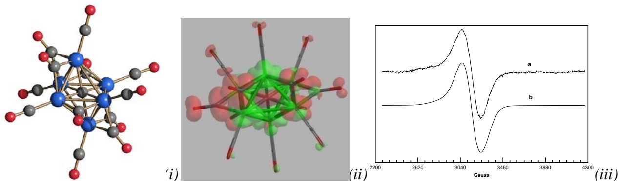
Fig. 4. (i) Molecular structure of [\text{Co}_6\text{C}(\text{CO})_{12}]^{3-} (blue, Co; red, O; grey, C); (ii) DFT calculated spin density surface ( 0.002 \text{ electron/au}^3 ) of the [\text{Co}_6\text{C}(\text{CO})_{12}]^{3-} cluster (red, negative spin density; green, positive spin density); (iii) X band EPR spectrum of [\text{NMe}_3(\text{CH}_2\text{Ph})_3][\text{Co}_6\text{C}(\text{CO})_{12}] \cdot 4\text{MeCN} in MeCN solution registered at 203 K: (a) experimental and (b) simulation. Reproduced with permission from ref. 78.
