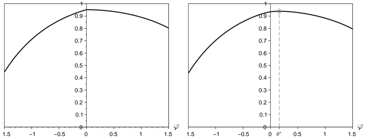
(a) \varphi \mapsto U(V_T^\varphi | V_T^0) .
