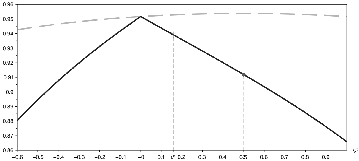
(a) \varphi \mapsto U(V_T^\varphi | V_T^0) .
