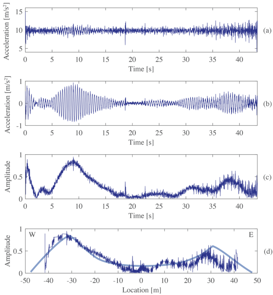
Figure 9 Steps of the procedure for a data sample: (a) vertical acceleration, (b) filtered signal, (c) filtered amplitude, (d) reconstructed sample shape
