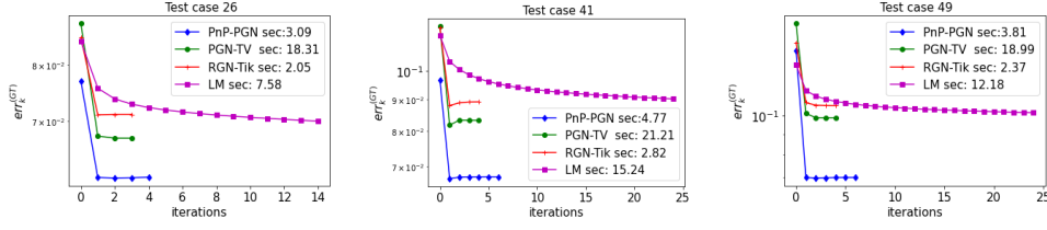
FIGURE 2. Relative error (46) between x^{GT} and the approximated solutions obtained by the algorithms PnP-PGN, PGN-TV, RGN-Tik, and LM, for three different test cases.
