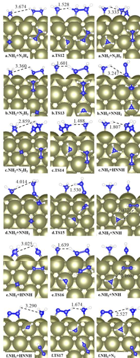
Figure 10. Top and side views of the initial, transition and final states for \text{N}_2\text{H}_x ( x= 1-4 ) attacked by \text{NH}_2 . (a) \text{N}_2\text{H}_4 to \text{N}_2\text{H}_3 , (b) \text{N}_2\text{H}_3 to \text{NNH}_2 , (c) \text{N}_2\text{H}_3 to \text{HNNH} , (d) \text{NNH}_2 to \text{NNH} , (e) \text{HNNH} to \text{NNH} and (e) \text{NNH} to \text{N}_2 . All inset distances are in \text{\AA} . Blue spheres represent N atoms, white is hydrogen, and Ir is the large green sphere.
