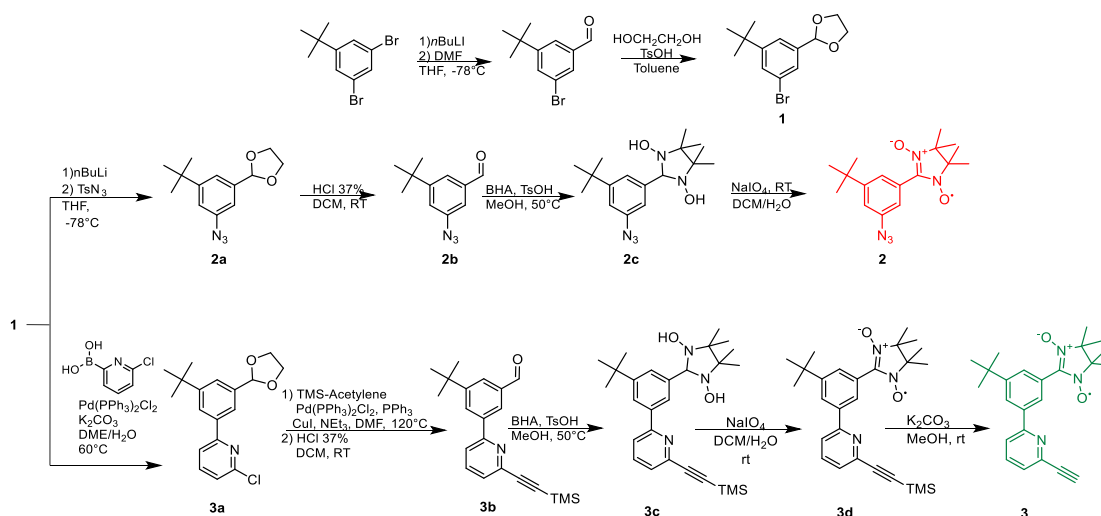
Scheme 1S. Synthesis of the spin-labelled half-axes.
