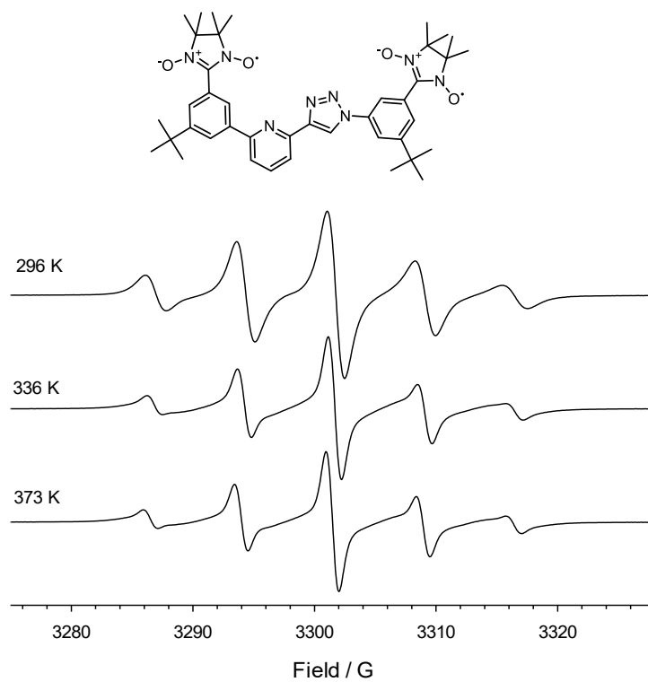
Figure S38. EPR spectra of Axle-3 in tert -butylbenzene at different temperatures.
