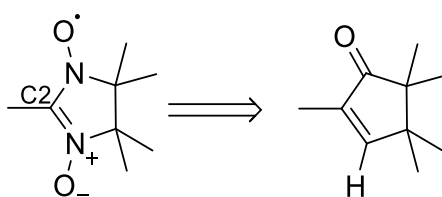
Figure S40. Simplified model employed for dynamic simulation of nitronyl nitroxides.
