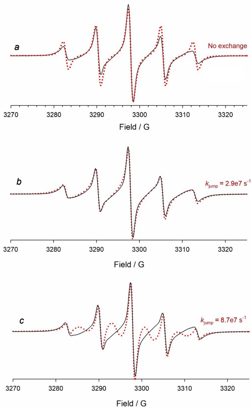
Figure S39. EPR spectrum of Rotax-3 in MeCN at 298K (black line) and theoretical simulations (red dotted lines) obtained in the absence of exchange (spectrum a), with a rate of exchange equal to 2.9 \times 10^7 \text{ s}^{-1} (spectrum b) and 8.7 \times 10^7 \text{ s}^{-1} (spectrum c).
