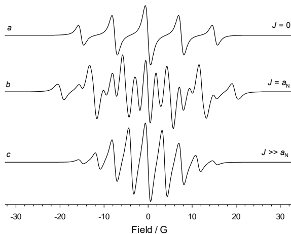
Figure S36. Theoretical spectra for a symmetric bis(nitronyl nitroxide) calculated by using a_N = 7.6 G and (a) J = 0 ; (b) J/g\mu_b = a_N ; (c) J \gg a_N .
