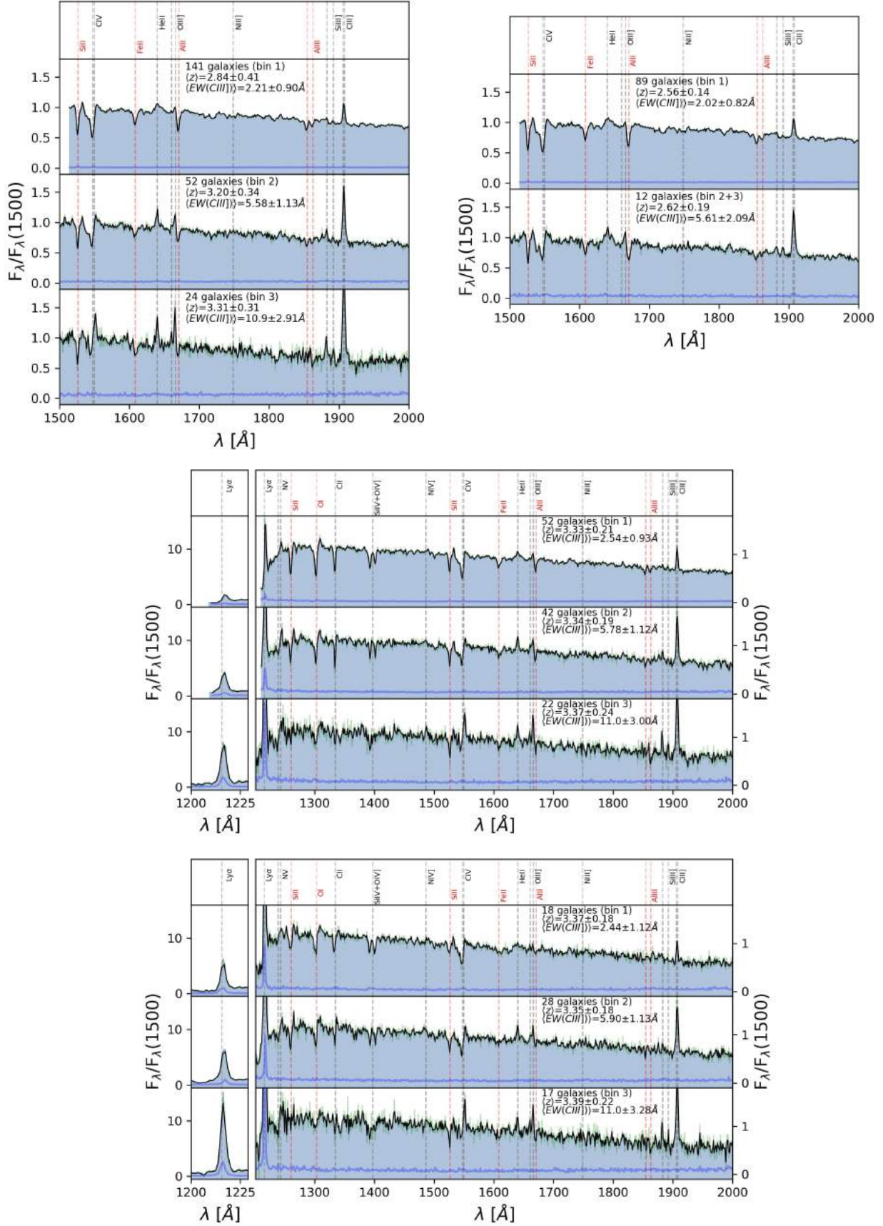
Fig. B.4. Stacks by EW(CIII]). Left to the right on top row: Stack A, Stack D. Middle row: Stack B. Bottom row: Stack C. In each panel, the green faint line is the stack spectrum with the \sim 0.6 \text{ \AA}/\text{pixel} sampling, while the black one is with \sim 1.2 \text{ \AA}/\text{pixel} . The blue line in the 1\text{-}\sigma error spectrum. The vertical lines mark known UV lines. Information about the number of galaxies, the mean redshift and the mean parameter are included in each panel.
