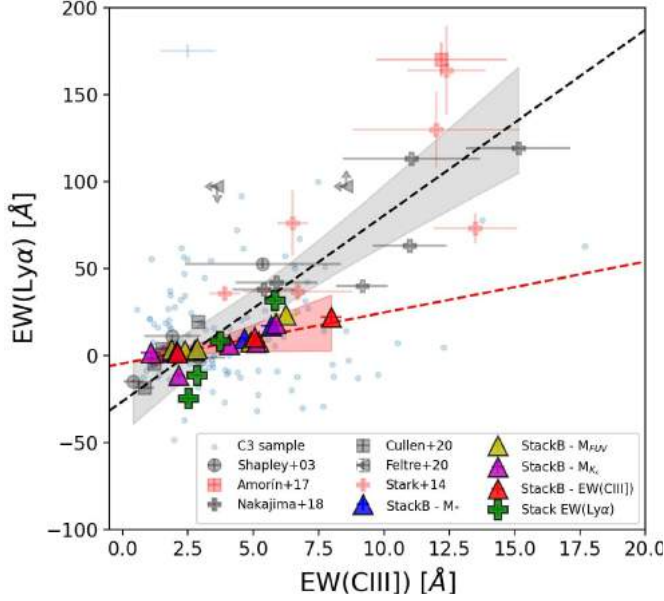
Fig. 13. EW(\text{Ly}\alpha) – EW(\text{CIII])} relation. The results from stacks B are represented by the triangle symbols, with different color depending on the parameter used for stacking: blue for stellar mass, yellow for FUV luminosity, magenta for K_s luminosity, red for EW(\text{CIII])} , and green for EW(\text{Ly}\alpha) . Individual galaxies with measured \text{Ly}\alpha from the C3 sample are the small blue circles with their typical errors on the upper left. Previous results from literature at similar redshift are also displayed from stacking (Shapley et al. 2003; Amorín et al. 2017; Nakajima et al. 2018b; Cullen et al. 2020; Feltre et al. 2020) and individual objects (Stark et al. 2014). Dashed black line is the best fit in Eq. (1) including our stacks and the sample from literature. Dashed red line is the best fit in Eq. (2), including just our stacks.
