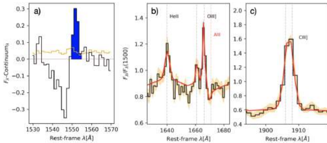
Fig. 9. Emission-line flux and EW measurements in the stack by EW(Ly\alpha) > 20 . Panel a: continuum-subtracted spectrum. The orange line shows the error spectrum ( 1\sigma ). The blue shaded region are the pixel integrated for the CIV line. Panels b and c: red line is the linefit fitting for the spectrum. The orange shaded region shows 1\sigma uncertainty of the stacked spectrum.
