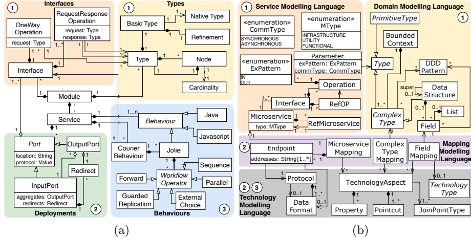
Figure 1: Core meta-models of Jolie (a) and LEMMA (b).
