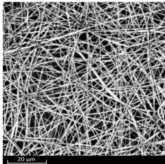
Fig. 3 SEM view of the nanofibrous layer
