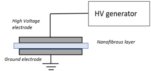
Fig. 4 Polarization setup
