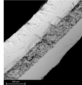
Fig. 7 SEM cross section view of the sensor
