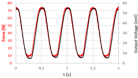
Fig. 9 Piezoelectric response in the time to a sinusoidal stress, f=2\text{Hz} ( V_{pk-pk}=48\text{ mV} , F_{pk-pk}=65\text{ N} )
