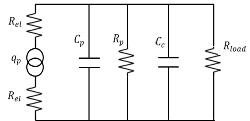
Fig. 8 Equivalent circuit of the realized piezoelectric sensor
