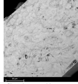
Fig. 6 SEM view of nanofibers integrated in epoxy resin and polyurethane rubber
