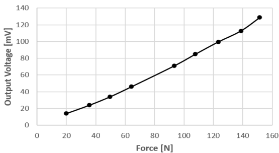
Fig. 10 Piezoelectric response at different sinusoidal stress, f=2\text{ Hz} .
