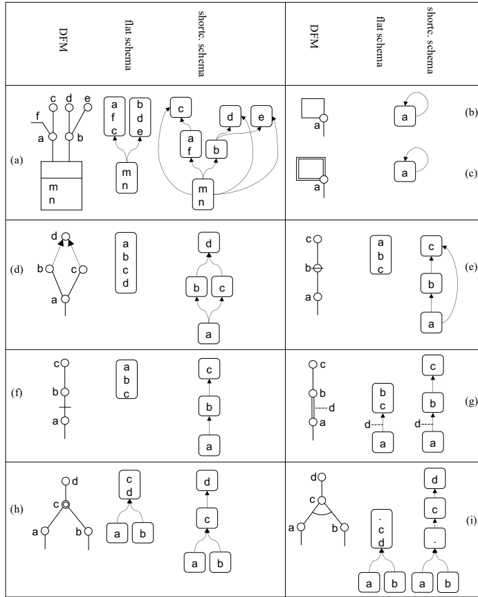
Fig. 7. Graph-based design alternatives for each multidimensional element
