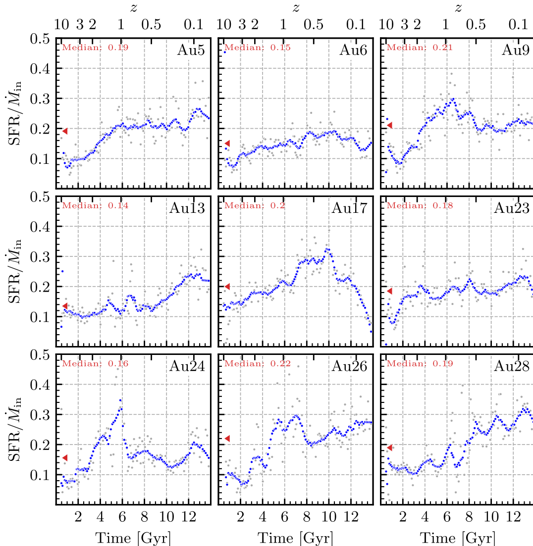
Figure 8. Ratio between the SFR and the inflow rate for the raw data of each galaxy (black dots). Blue dots indicate the same ratio but for the smoothed curves (trend) shown in Fig. 6. The red triangle marks the median value indicated in the top left corner. Ratios vary in the range 0.1–0.3 and are, in general, higher at late times.
