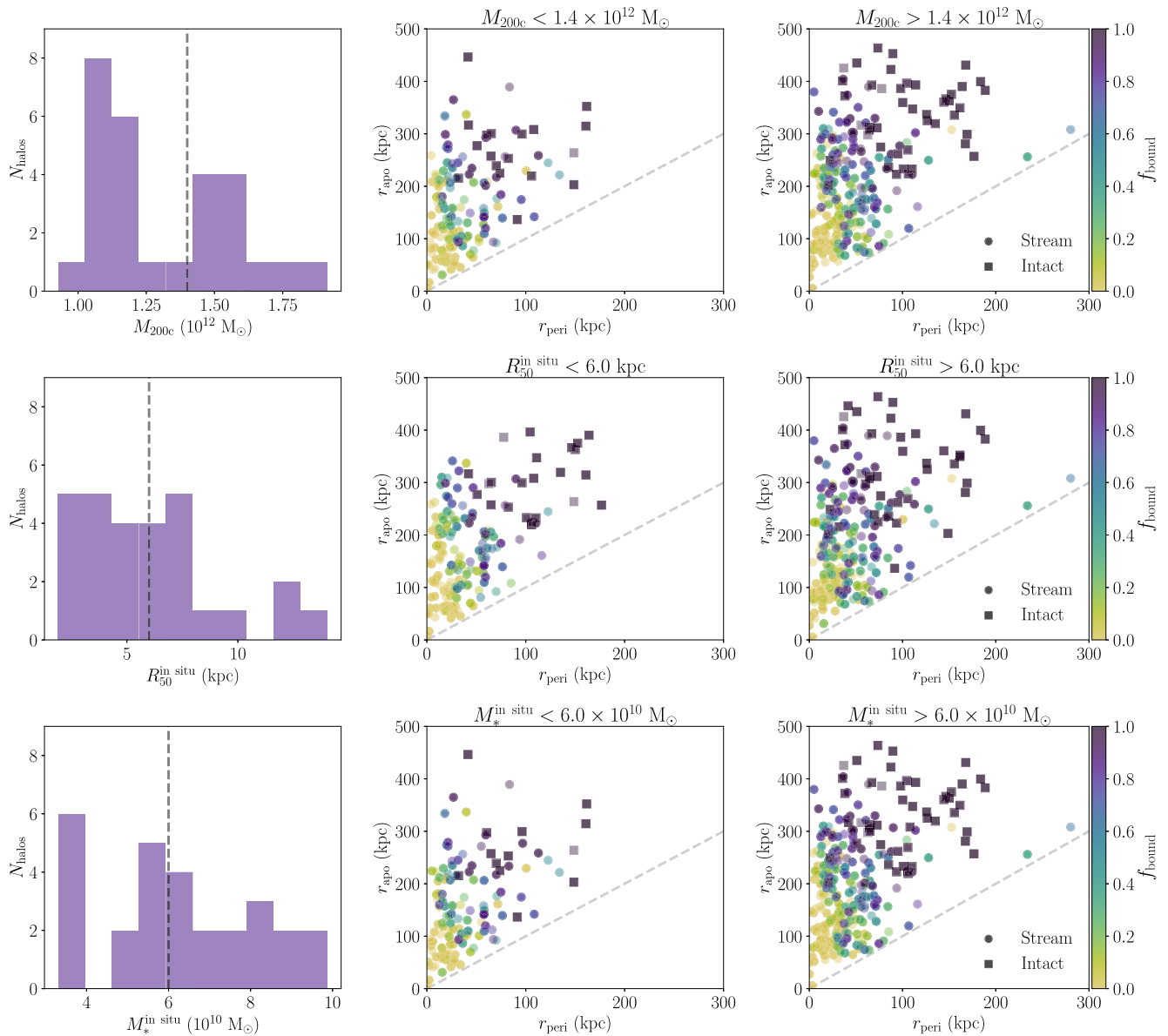
Figure 10. Pericentres and apocentres of intact satellites and stellar streams around 28 level 4 host galaxies binned by host galaxy properties. In the top row, galaxies are binned by host halo mass ( M_{200c} ). The histogram on the left shows the distribution of host masses across the 28 simulations and the grey dashed line indicates that value on which the sample is split. The panels in the centre and right show the pericentres and apocentres of satellites around galaxies in each mass bin. The middle row shows the same for disc size ( R_{50}^{\text{in situ}} , defined as the spherical radius which encloses 50 per cent of in situ stellar mass), and the bottom row shows the distribution across host in situ stellar mass ( M_*^{\text{in situ}} ).
