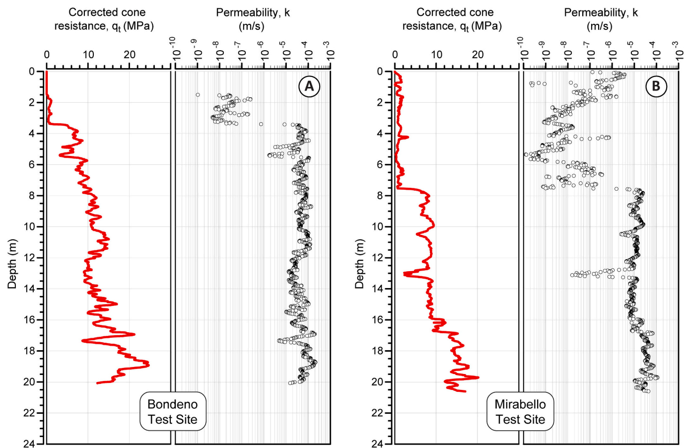
Fig. 6. CPTU-based predicted values of permeability for (a) the Bondeno blast test site subsoil and (b) the Mirabello blast test site subsoil.
