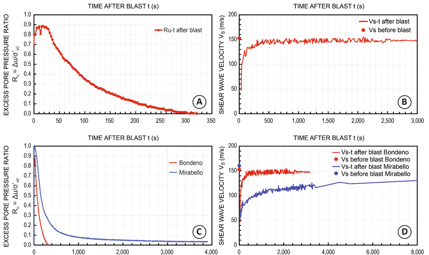
Fig. 10. R_u (PPT6, 5.84 m depth) (a) and V_s (SDMT blast, 6.10 m depth) (b) profiles vs. time (Bondeno); comparisons between R_u (c) and V_s (d) vs. time (Bondeno PPT 5.84 m- SDMT blast 6.10 m & Mirabello PPT 7.5 m SDMT 7.25 m).
