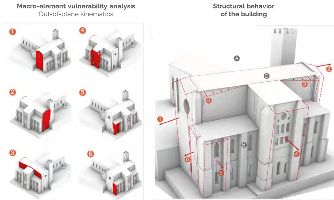
Figure 12. On the top, TLS point cloud of the Basilica of San Domenico in Siena: identification of the investigated masonry walls and the reference system. On the bottom, an analysis of macro-elements and an interpretation of the structural behavior of the transept of the Basilica of San Domenico in Siena.
