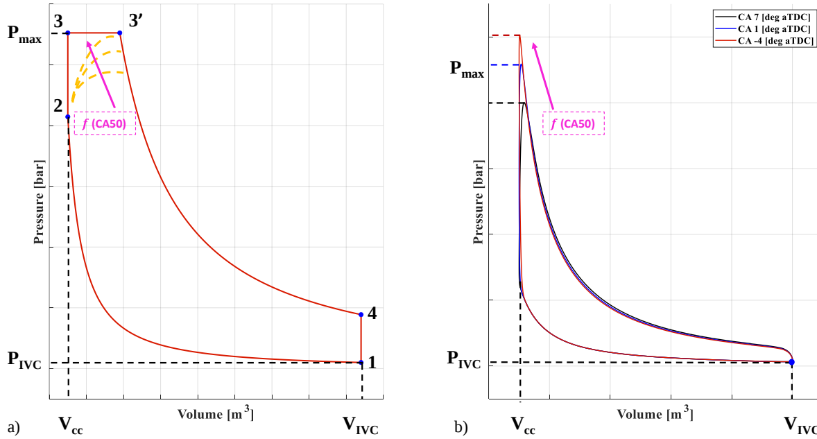
Figure 4. Indicator diagram: a) effect of CA50 on combustion process of the ideal Seiliger-Sabathe cycle, b) effect of CA50 on the real combustion process of the 4-cylinder turbocharged SI engine
