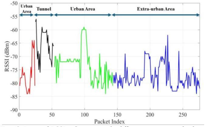
Fig. 13. Retrieved RSSI with respect to the different environments that have been crossed by the train, with the two modules placed outside it at a distance of about 75 m.
