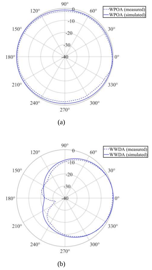
Fig. 10. Normalized radiation patterns of (a) WPOA (for an elevation angle of 25^\circ with respect to the xy plane) and (b) WWDA (in the xy plane).
