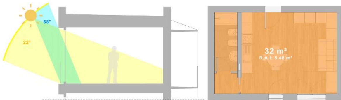
Figure 4. Sample dwelling unit in section and plan. Elaborated by L. Pataconi and M. Stefanini.
