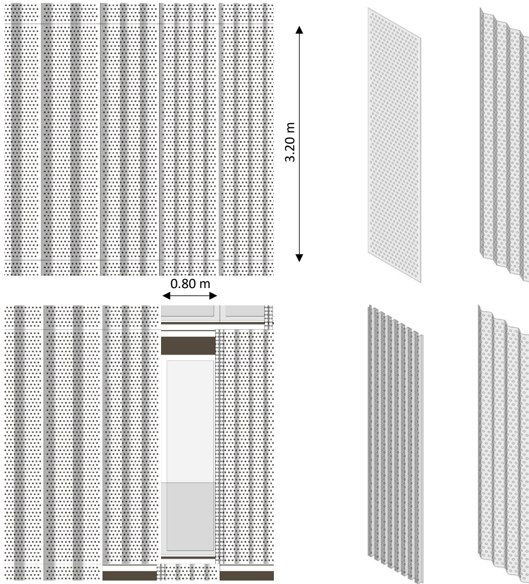
Figure 5. Layout drawings of the shading system and override position (bottom) with alternative panel sections from flat sheet to wavy sheet.
