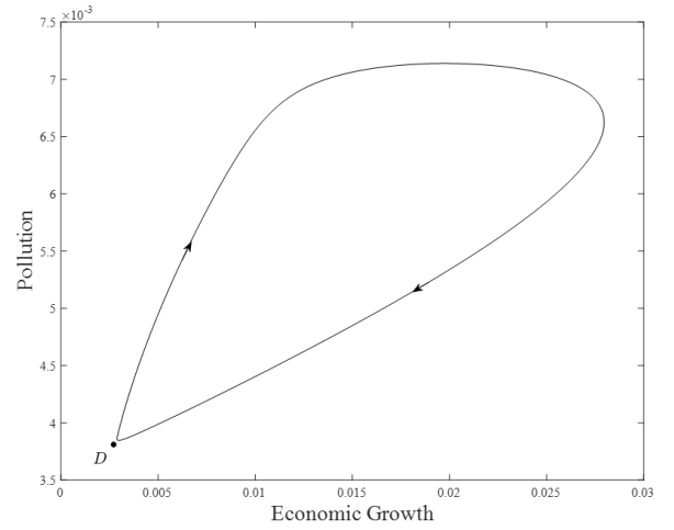
7b. \pi_k = 0.5689851
