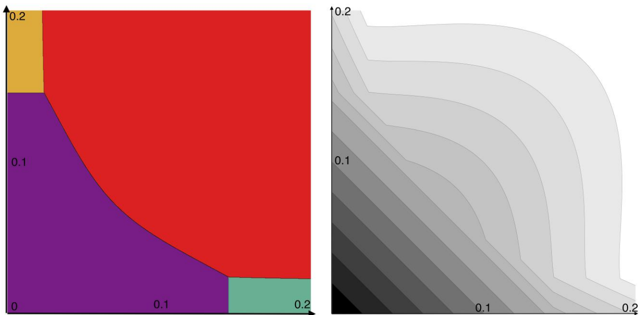
Figure 1. (Color online) Optimal Payment Network (Left) and Its Cost (Right) if Alice Pays Bob at Rate \lambda_1 (Horizontal Axis, from 0 to 0.2), and Bob Pays Alice at Rate \lambda_2 (Vertical Axis, from 0 to 0.2 in Number of Annual Transactions) with Round-Trip Transaction Cost B = 1 and Interest Rate r = 1\%
