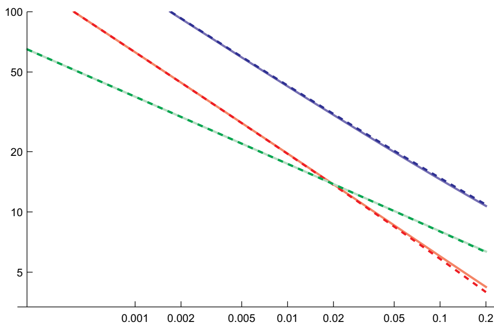
Figure 4. (Color online) Exact (Solid) and Asymptotic (Dashed) Cost (Vertical) of Unidirectional (Red or Light Grey, (2) vs. (7)), Bidirectional Symmetric (Green or Medium Grey, Minimum of (3) vs. (8)), and Bidirectional Asymmetric (Blue or Dark Grey, Minimum of (3) vs. (13)) Channels Against the Interest Rate (Horizontal), for B = 1, \lambda_1 = 1 , and (for the Blue Plot) \lambda_2 = 5
