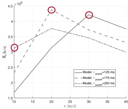
Fig. 15: Average cluster throughput for the dynamic case when varying v and \tau_{pusch} ; \bar{n} = 1000 .
