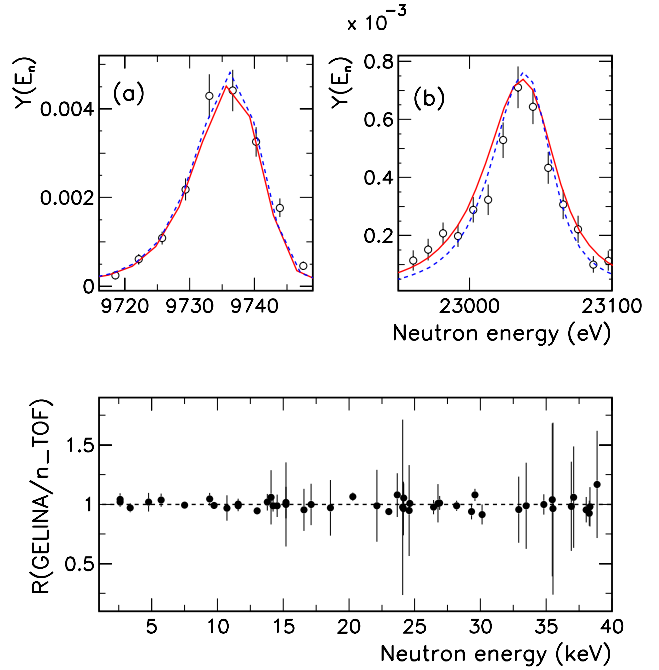
Fig. 5 (Color online) Upper panels: experimental capture yields obtained at n_TOF. The results of \mathcal{R} -matrix fits (with the as \Gamma_\gamma free parameter) to these yields are represented by a blue dashed line. The red full line is the theoretical yield using the resonance parameters derived from the GELINA data; see text for details. Lower panel: Ratio of the capture kernels extracted from the n_TOF (SAMMY code) and GELINA (REFIT code) data as a function of the resonance energy.
