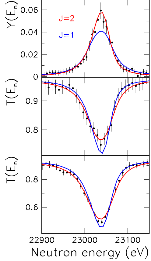
Fig. 3 (Color online) Upper panel: experimental capture yield obtained at GELINA; Lower panels: Results of transmission measurements performed with the 2 squared layers (middle) and the thick disk + 2 squared layers (lowest panel) ^{89}\text{Y} samples, see Tab. 2. The results of \mathcal{R} -matrix fits are included. See text for the details.
