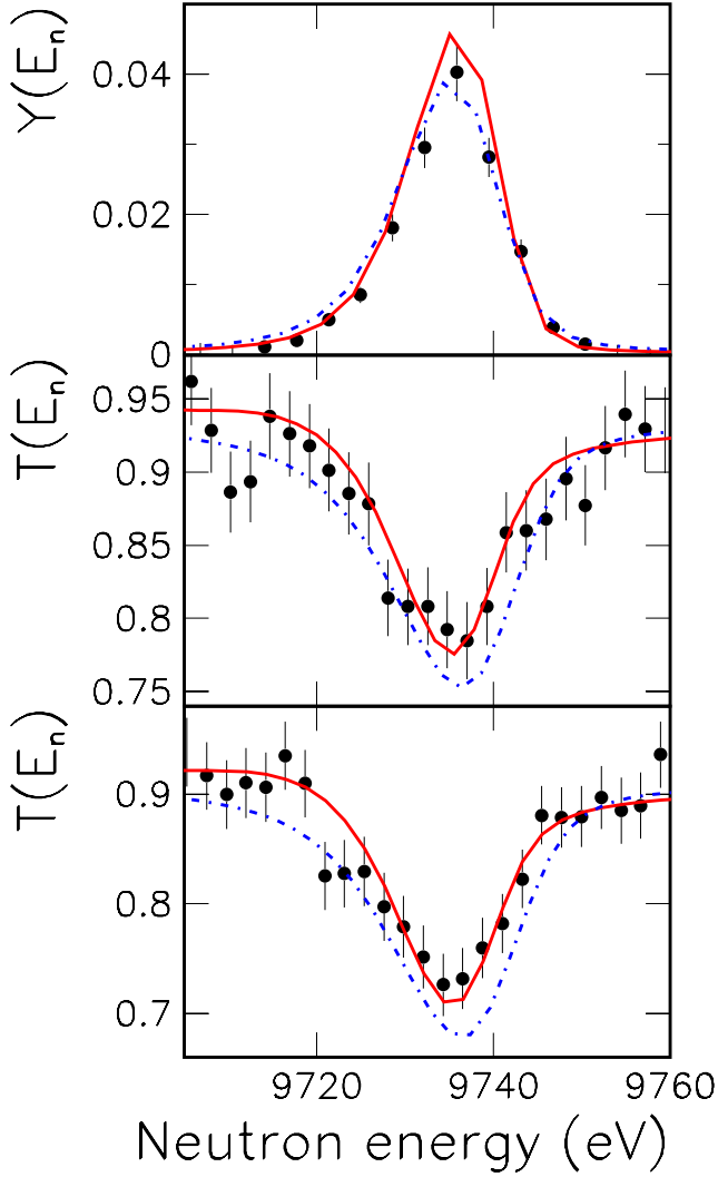
Fig. 2 (Color online) Upper panel: experimental capture yields obtained at GELINA; Lower panels: results of transmission measurements performed at GELINA with the thick disk + 2 squared layers (middle) and the 7 squared layers (lowest panel) ^{89}\text{Y} samples, see Tab. 2. The results of \mathcal{R} -matrix fits are included. Full red lines refer to a fit with \ell = 0 , J = 0 ; blue dash-dotted lines to a fit with \ell = 1 , J = 0 .
