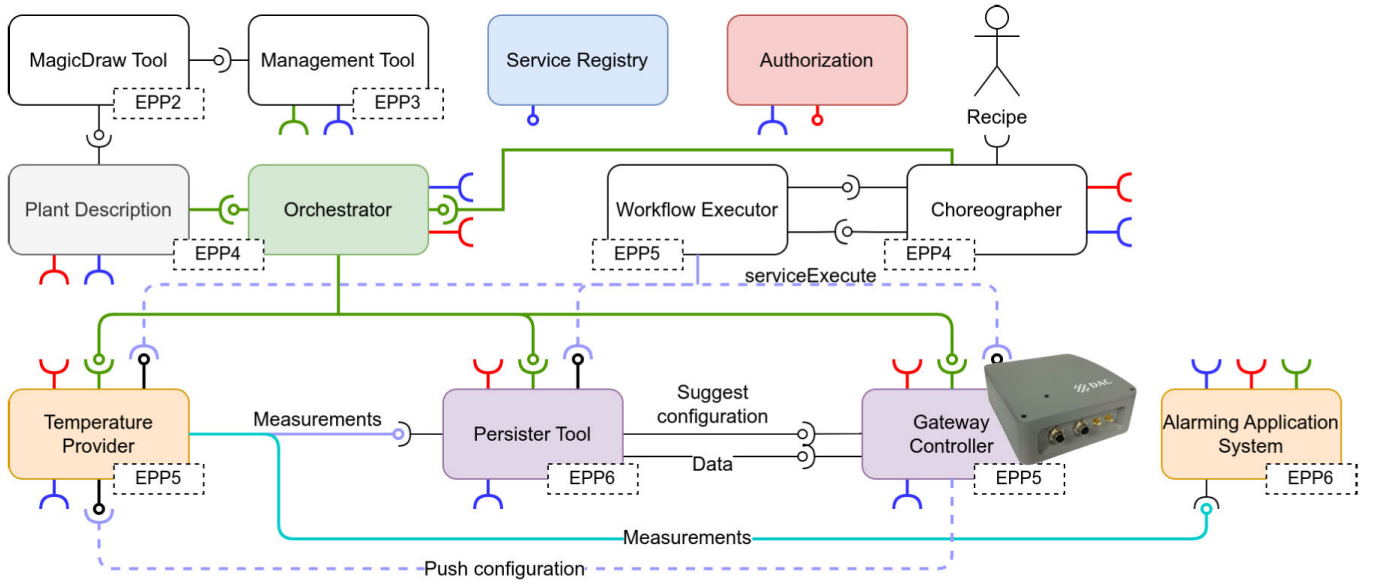
Fig. 4. Architecture of the demonstrator system with the workflow choreographer at the adoption level 4. EPPX describes the number of engineering phase to which the tool or interaction is attributed (see Figure 2). It is assumed that all tools are orchestrable and choreographable.
