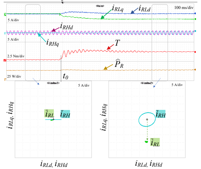
Fig. 16 - Locked rotor behavior of the drive during a step change of the torque command while the power delivered to the rotor loads is 100 W and the torque ripple suppression scheme is activated. Waveforms of the torque T (2.5 Nm/div) and average rotor power \hat{P}_R (25 W/div) d-q components of the low- and high-frequency rotor currents (5 A/div) and their respective trajectories in the d-q plane.
