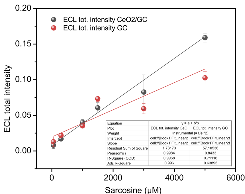
Figure 4. The ECL total intensity as a function of sarcosine concentration is measured on bare GC and CeO 2 /GC electrodes in 200 mM PBS (pH 7.2) containing 10 μM Ru(bpy) 3 2+ . The error is represented as standard deviation (n=3).
