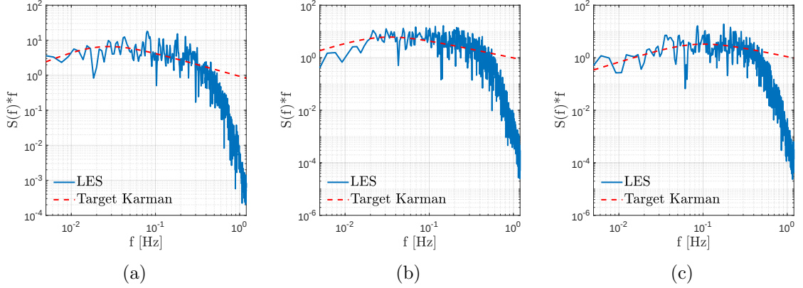
Fig. 6. Spectra of the velocity components measured at H_r : along-wind component (a), cross-wind component (b) and vertical component (c).
