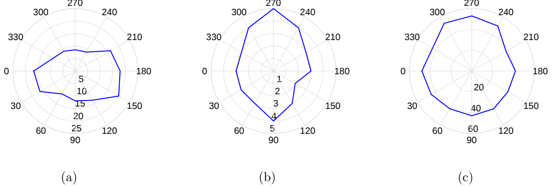
Fig. 10. Proper Orthogonal Decomposition of the pressure field: (a) energy of the first mode (percentage), (b) number of modes required to obtain 25% of total energy and (c) number of modes required to obtain 75% of total energy.
