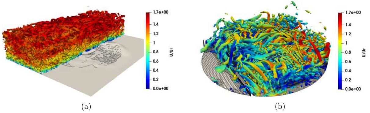
Fig. 7. Overview of the flow field by means of instantaneous Q-criterion iso-surfaces colored by U/U_r : (a) overall domain ( Q = 0 ) and (b) around the stadium at 120^\circ ( Q = 2 ).
