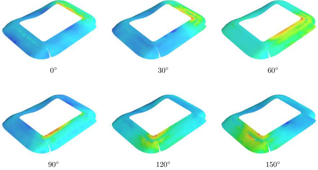
Fig. 9. Proper Orthogonal Decomposition, an overview of the first mode for angles up to 150^\circ (colorbar not reported as the POD modes are not defined in amplitude).
