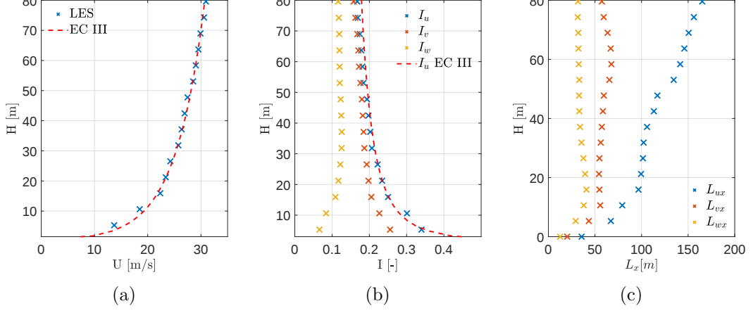
Fig. 5. Velocity profiles obtained from the empty domain test: (a) mean velocity profiles, (b) turbulence intensity profiles and (c) turbulence length scale profiles.
