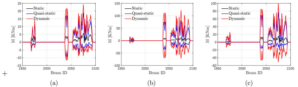
Fig. 21. Comparison between design envelopes for bending moments obtained from the static, quasi-static and dynamic components of the structure response: (a) 0^\circ , (b) 60^\circ and (c) 120^\circ .
