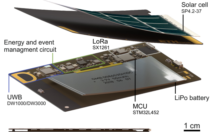
Fig. 4. Prototype of the designed self-sustainable indoor localization tag in the shape of an 85 mm \times 55 mm \times 2 mm business card.
