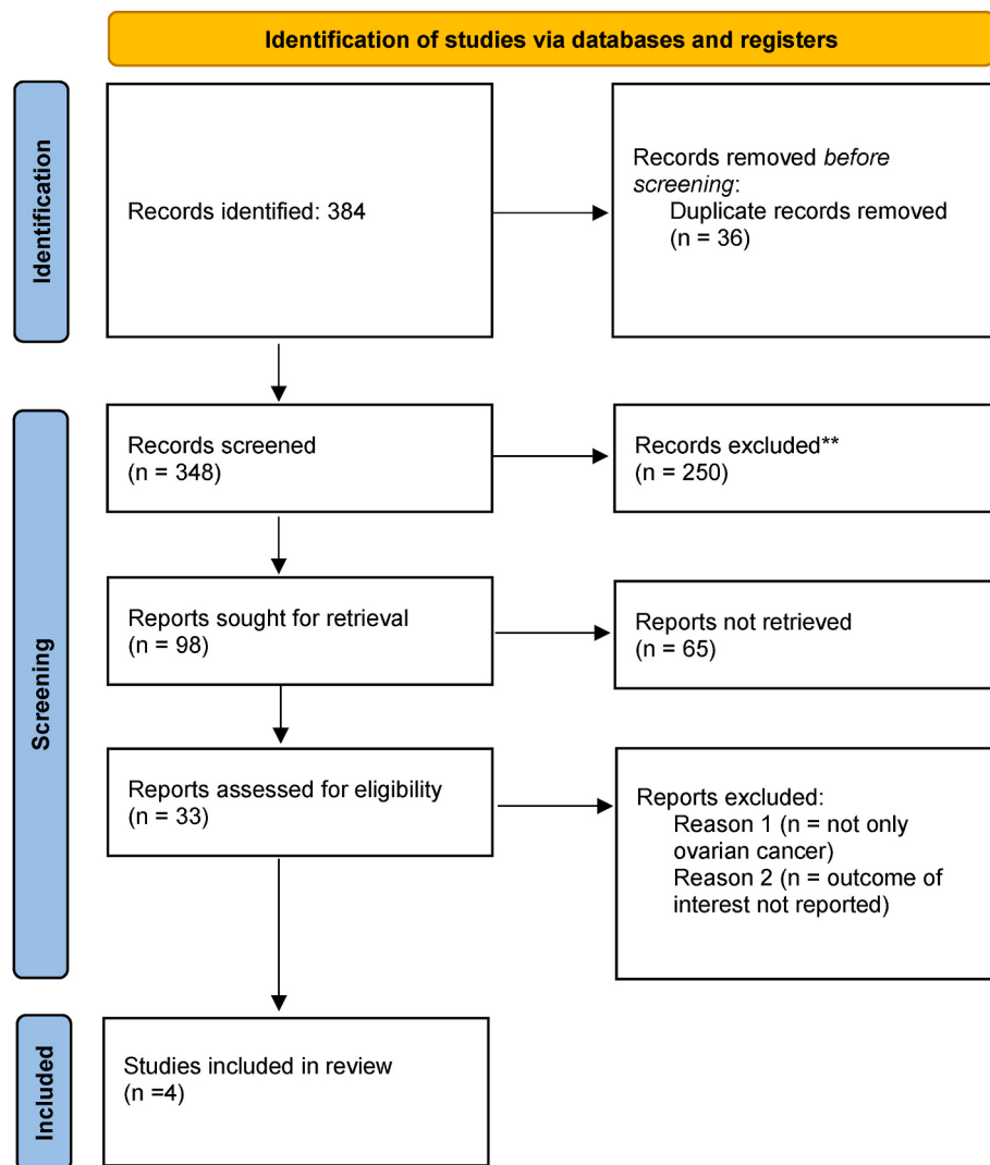
Fig. 1. PRISMA flowchart.
