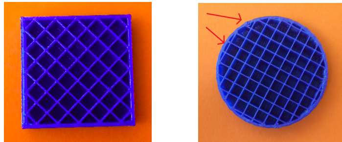
Fig. 5 Predefined square pattern for infill structure. In some parts the infill lines are very close to the boundary (external surface) of the object and/or the lines are very close to each other. As a consequence, the 3D printer hardly resolves the pattern, the extruder wastes time running for very short distance and the material already deposited melts again.
